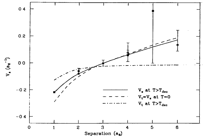
FIG. 1. The correlation function of spacelike Polyakov lines V_s(b) computed on 10^3 \times 6 and 6^3 \times 3 lattices is shown by squares and circles, respectively. The solid line is obtained by a fit with a function of the form V(b) = a/b + \sigma_s b + \text{const} . The dashed line is the V_t at T=0 , taken from Bowler et al. (Ref. 11). The dash-dotted curve is the V_t computed at 10^3 \times 6 and 6^3 \times 3 at T > T_{\text{dec}} . Everything is expressed in units of the lattice spacing a_6 of the 10^3 \times 6 lattice.
